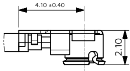
DETAIL B SCALE 8x CONNECTOR
